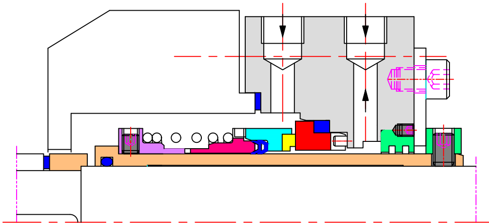
80 SERIES SINGLE SPRING MECHANICAL SEAL TYPE 8221 BD CARTRIDGE ARRANGEMENT WITH DIFFERENT API PLAN 11& 62
